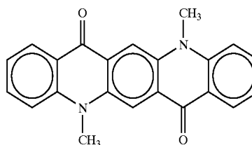
Quinacridone
